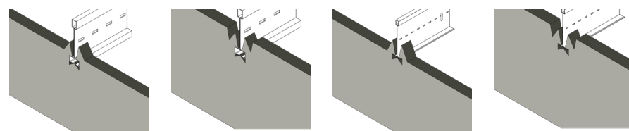
(FH) F-Snap High (FL) F-Snap Low (TH) T-Snap High (TL) T-Snap Low
