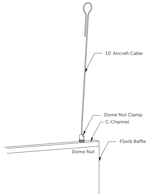
Dome Nut, Cable Gripper Kit, & C-Channel Installation
